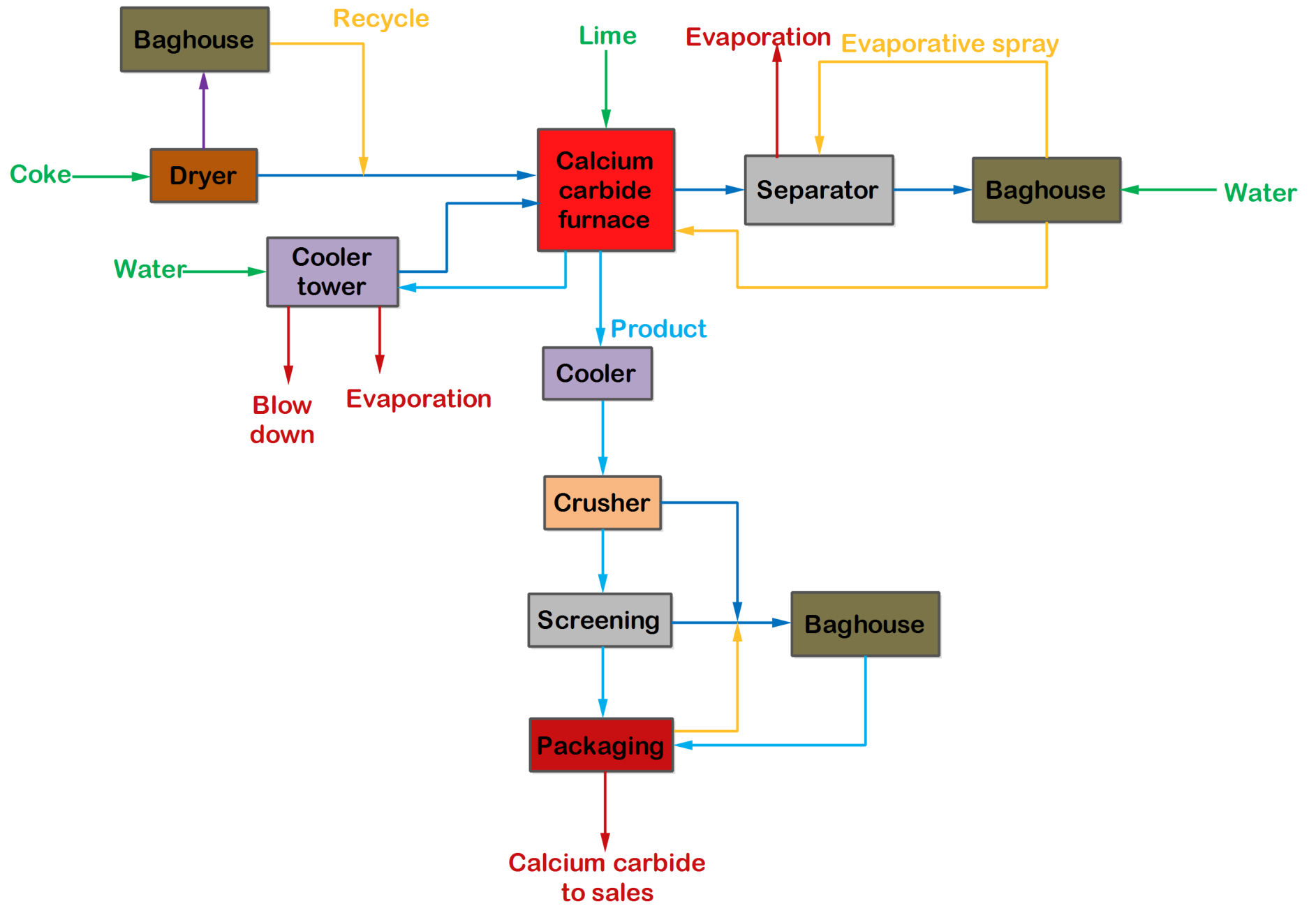
Figure: Manufacture of Calcium carbide using water
